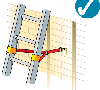
Figure 18c Tying at base
