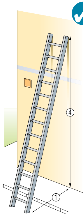
Figure 19 Ladder showing correct 1 in 4 angle (means of securing omitted for clarity)
