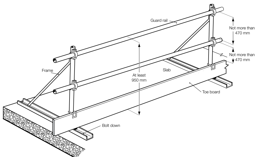
Figure 10 Guard rails and toe boards
