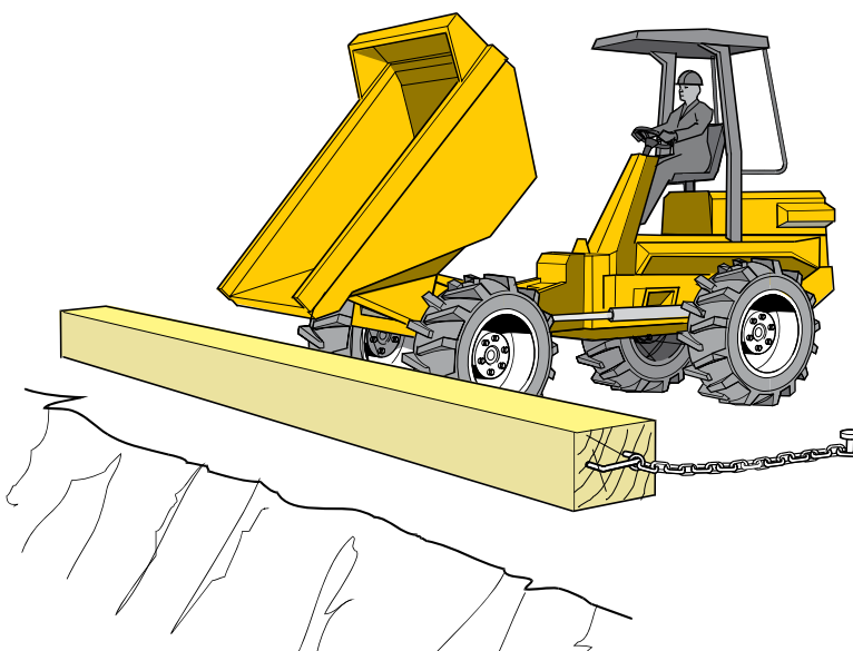
Figure 35 Take precautions, such as stop blocks, where vehicles tip materials into excavations
