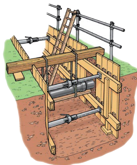
Figure 44 An excavation supported by timbering and props with guard rails (omitted from left-hand side for clarity) to prevent falls. Extended poling boards act as toe boards, safe access is provided by a tied ladder and exposed services are supported
