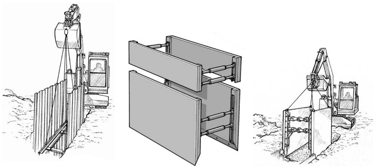
Figure 42 Proprietary trench boxes and hydraulic wallings allow trench supports to be put in place without requiring people to enter the excavation
