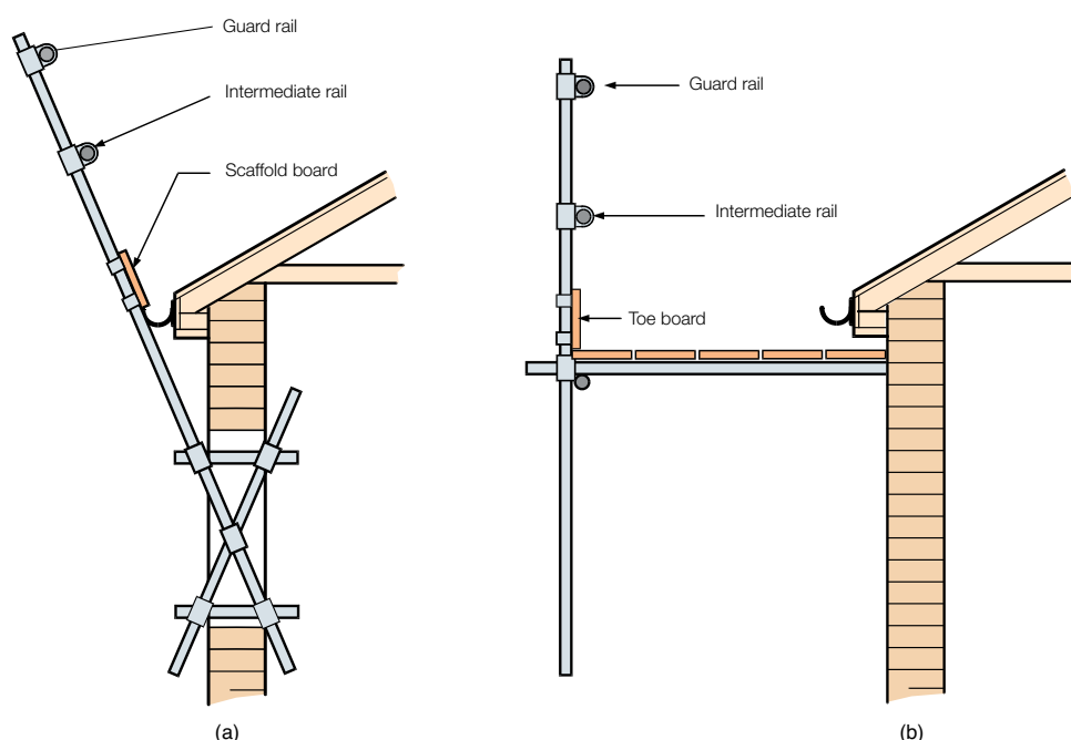
Figure 24 Example of flat-roof edge protection
