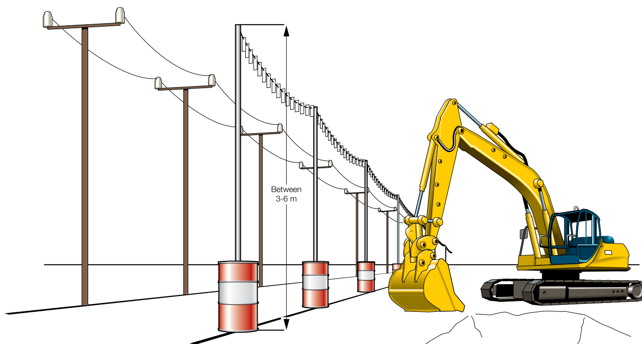
Figure 49 Ground-level barrier for plant working near an overhead power line
