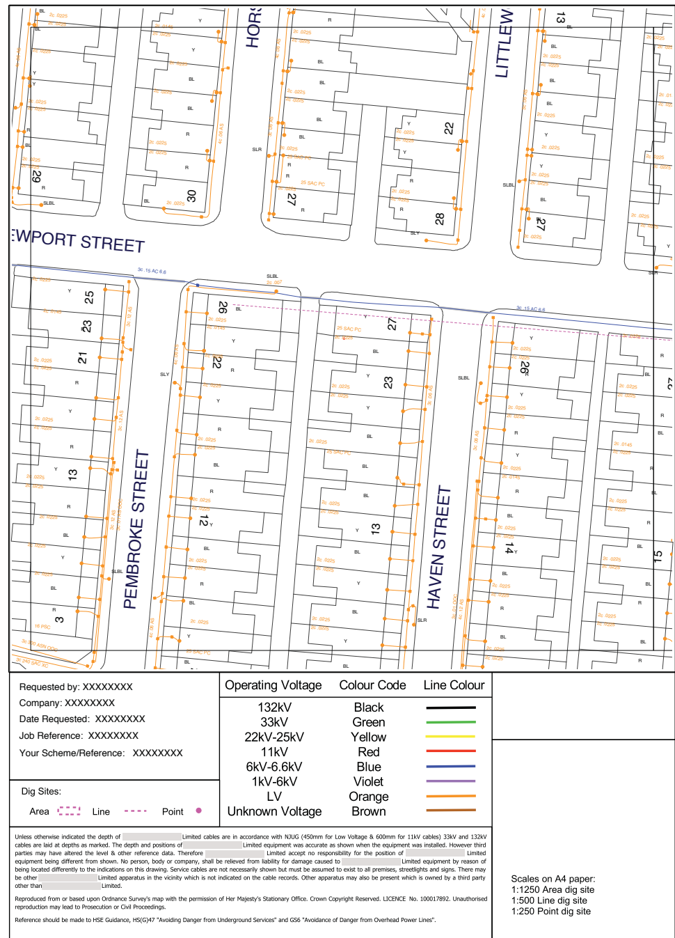
Figure 1 Example of an electricity plan
