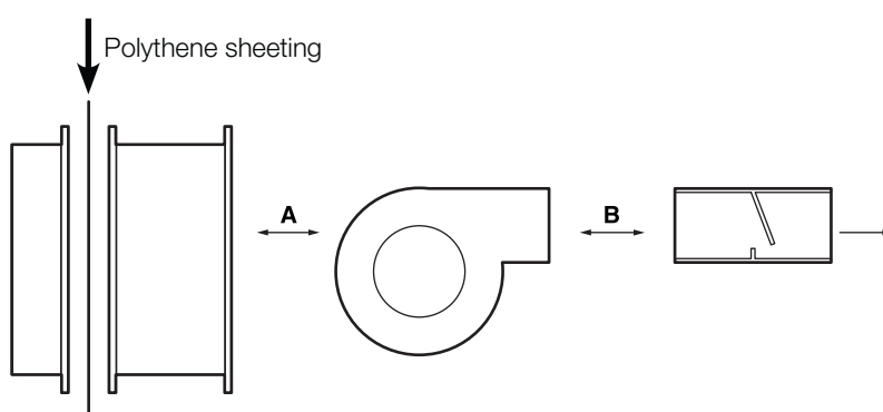
(c) Essential components of extract unit (Note: Components may be separated by flexible ducting at A or B in some designs)
