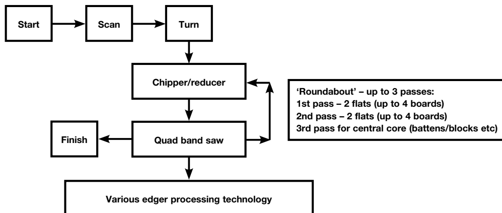
Figure 29 A typical mechanised sawmilling line
