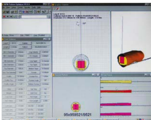
Figure 28 Display screen image of scanned log
