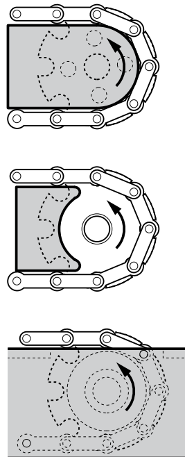
Figure 25 Example of chain/sprocket guard
