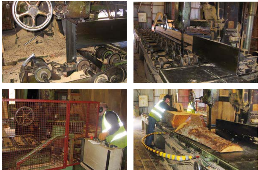
Figure 4a Travelling table log band saw (manual control) with inadequate safeguarding (top) and travelling table log band saw (manual control) after additional safeguarding has been fitted (below)
