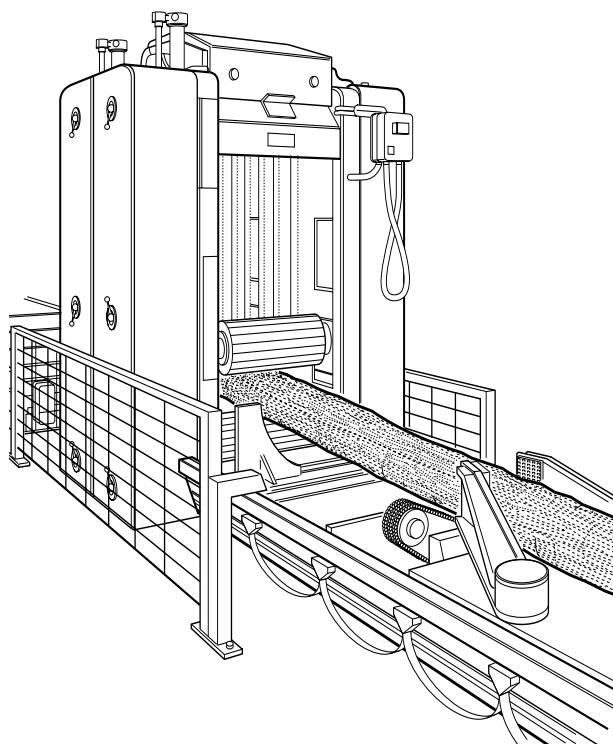
Figure 12 Frame saw (barrier along feed track not shown)
