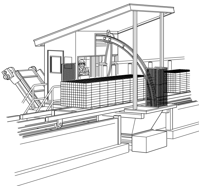
Figure 20 Static cross-cut chainsaw
