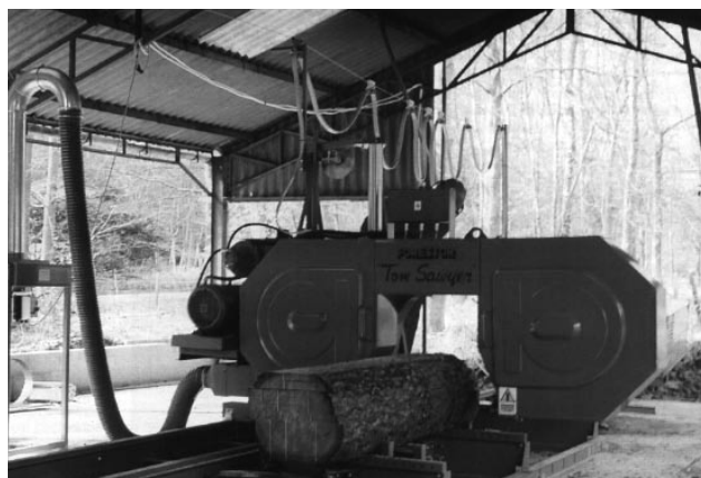
Figure 9 Moving head-rig log band saws
