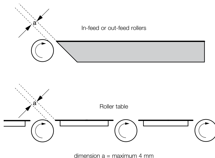
Figure 11 In-filling gaps between rollers and fixed parts in roller table
