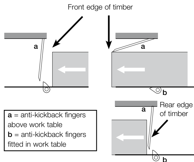
Figure 16 Anti-kickback fingers on multi-rip saws
