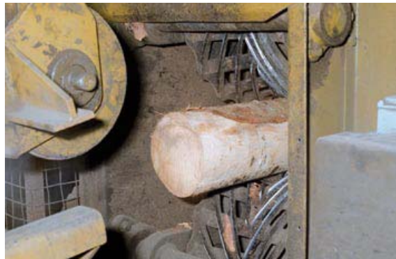
Figure 21 Through-feed debarker (guards not shown)
