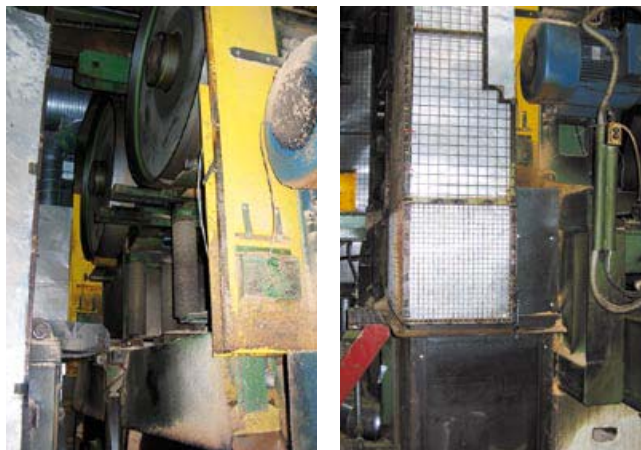
Figure 7 Open and closed fixed guarding around non-cutting area of band saw blade
