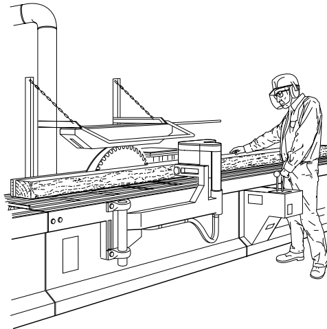
Figure 13 Travelling table circular log saw
