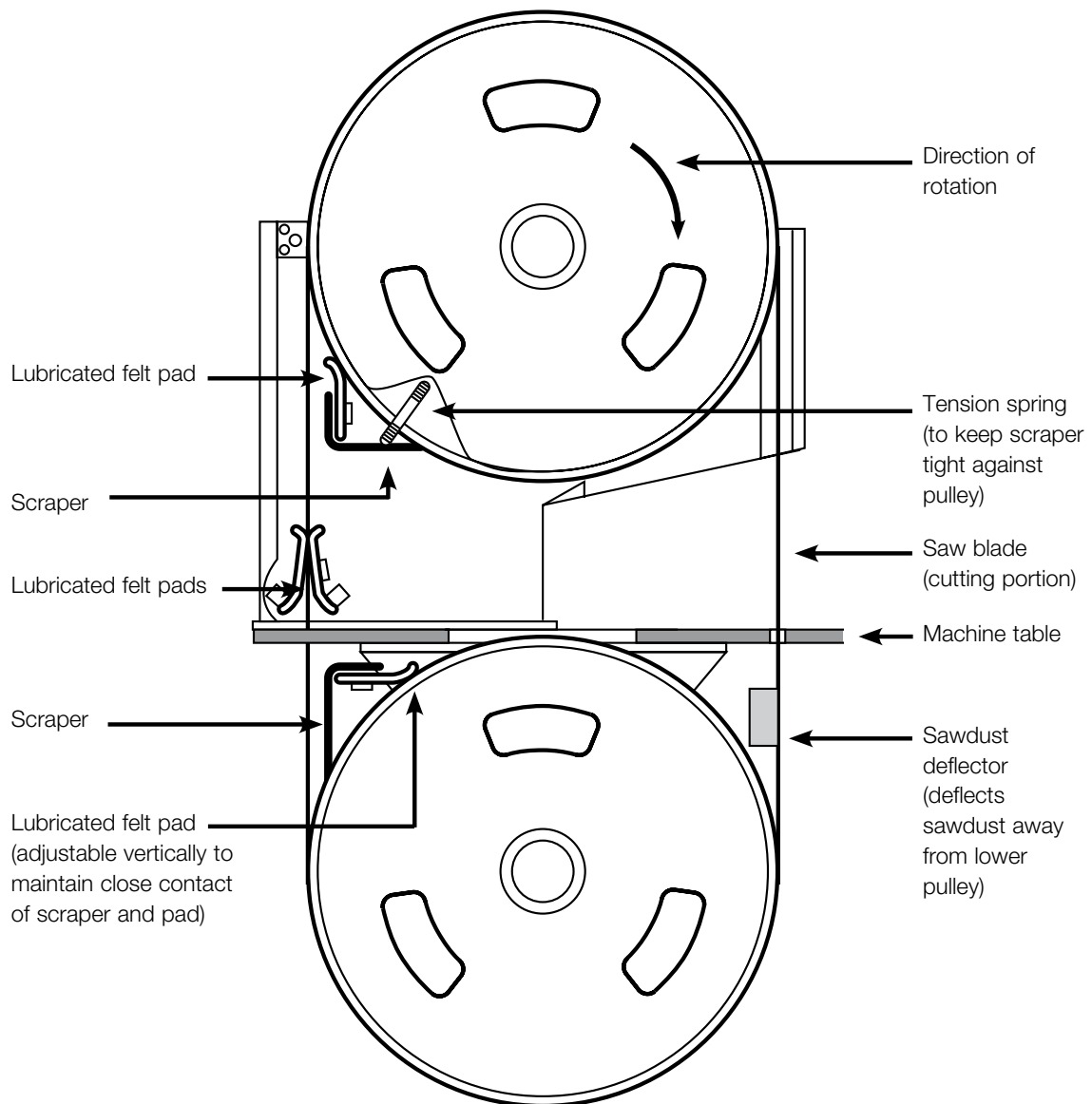
Figure 1 Band saw cleaning system (guards and machine detail not shown for illustration purposes)
