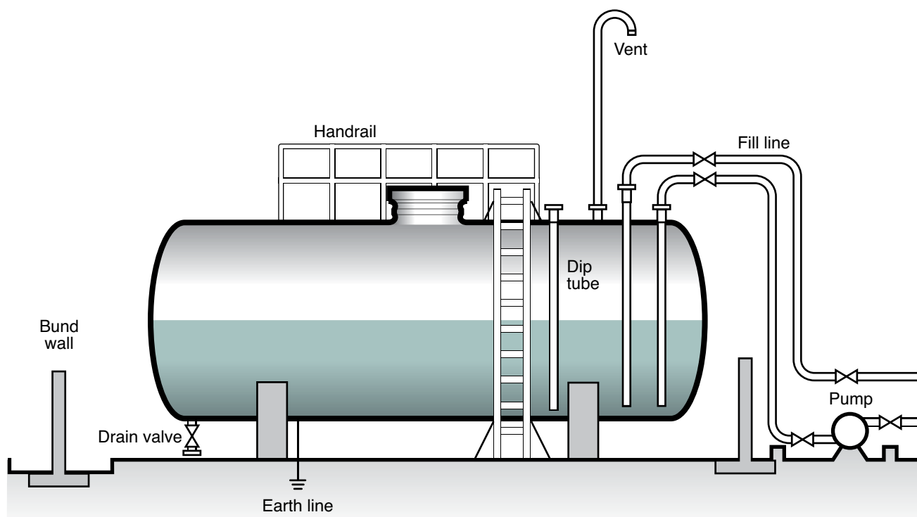
Figure 6 Typical horizontal storage tank (top discharge)
