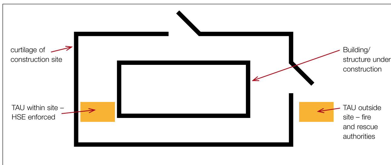
Figure 17 Fire safety requirements for stand-alone construction sites
