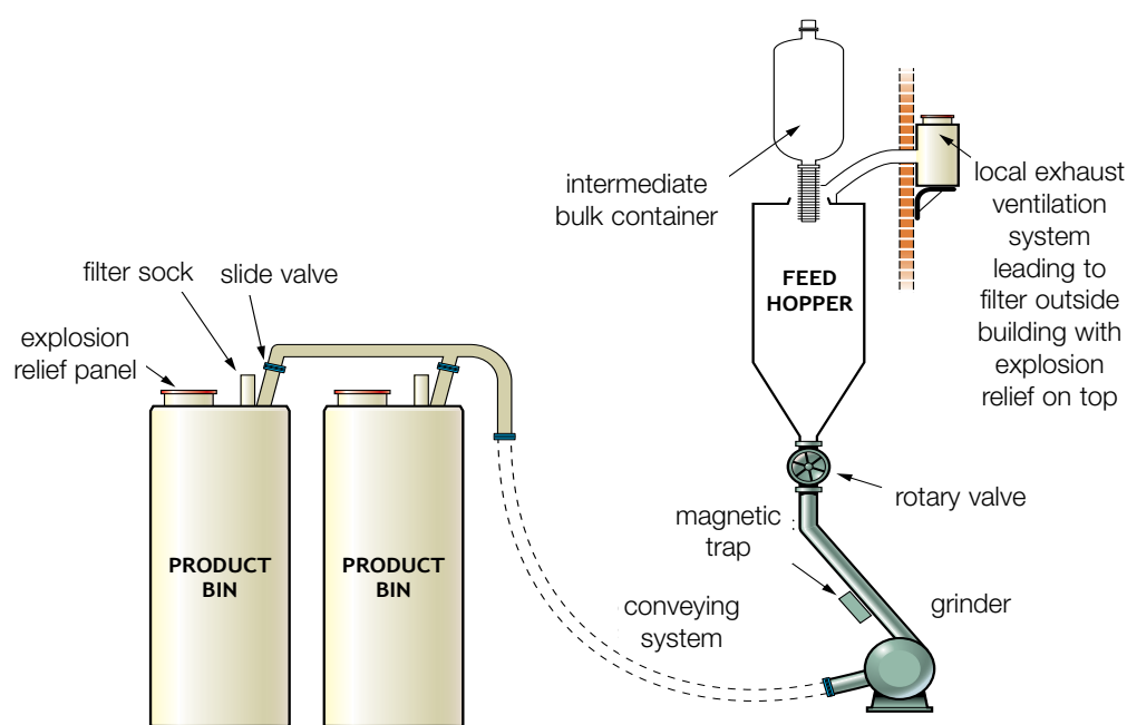
Figure 7 Simple grinding installation diagram
