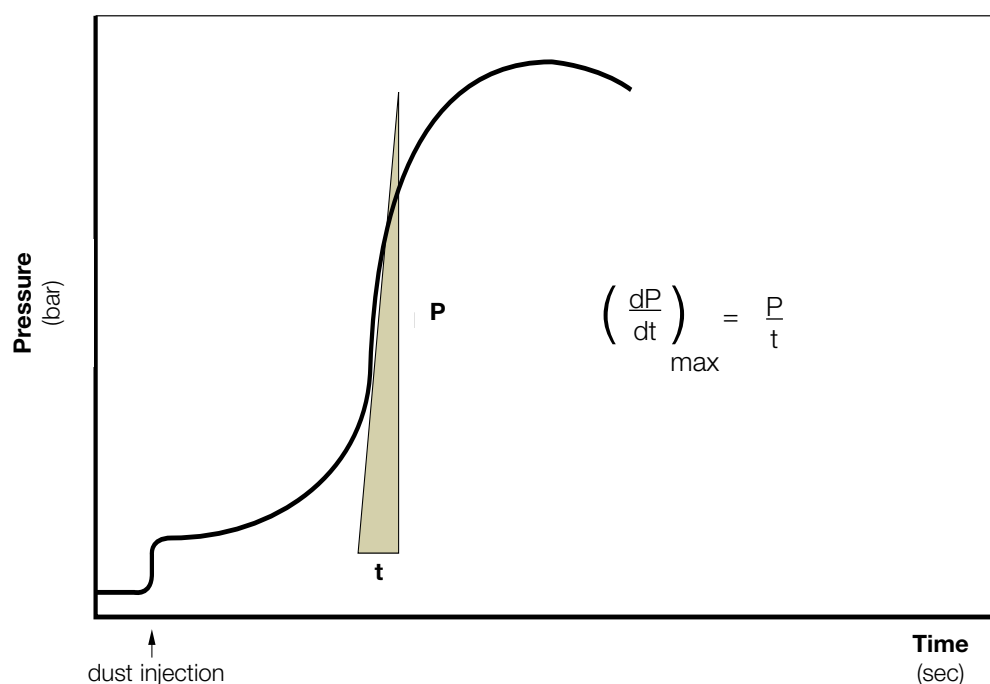
Figure 11 Typical trace from a dust explosion test
