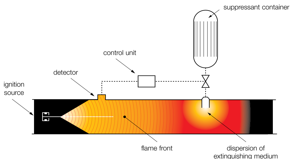
Figure 5 Suppressant barrier
