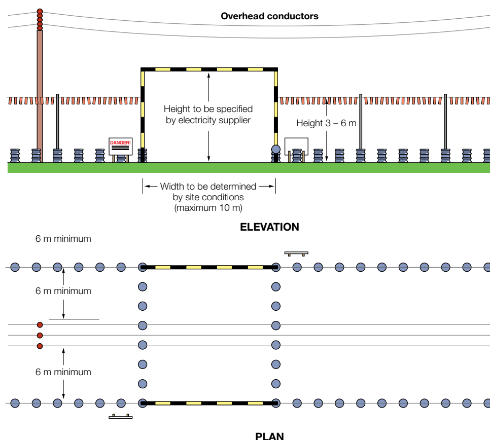
Figure 9 Diagram showing normal dimension for 'goal post' crossing points and barriers where plant is operating. Similar markings could be used to mark overhead power lines if long roof sheets or scaffold poles are being used
