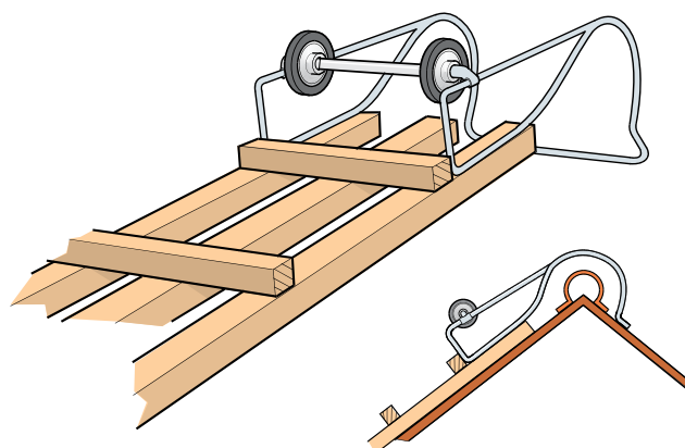
Figure 29 Roof ladder. The ridge iron should be large enough to be clear of the ridge tile
