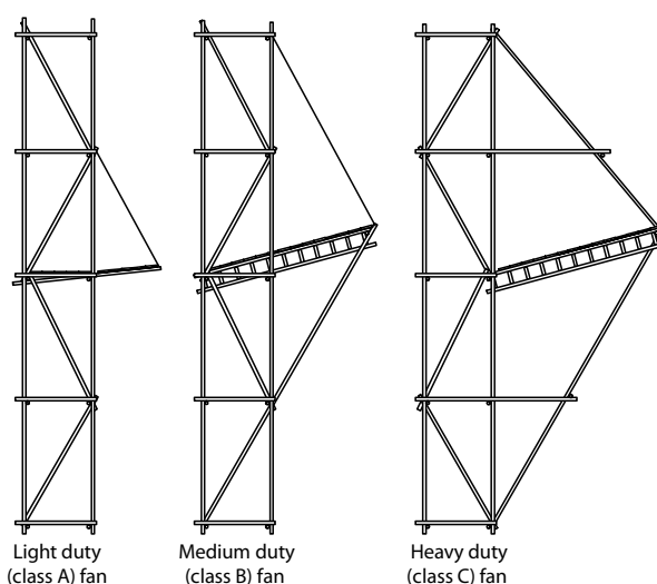
Figure 38(c) Scaffold fan classifications (Permission to reproduce extracts is granted by BSI)
