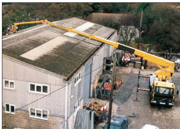
Figure 12 Powered access for inspecting a large fragile roof
